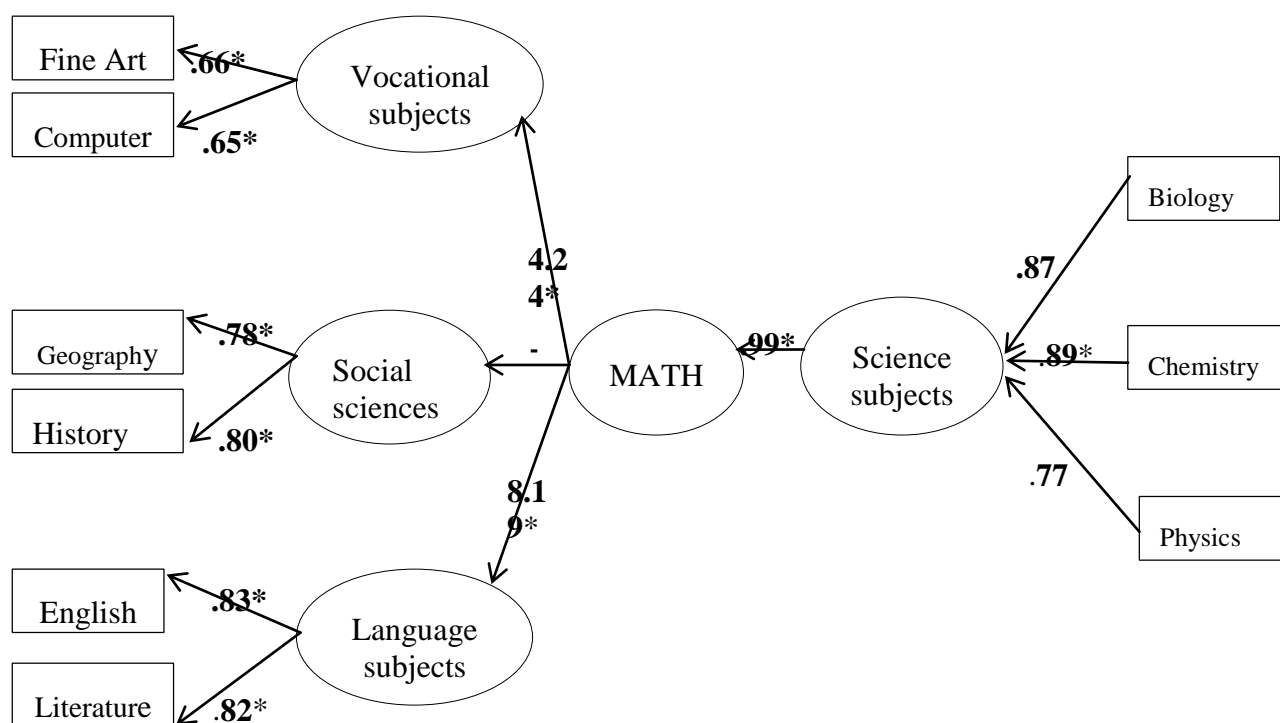
Figure 2: Structural equation model and significant standardized estimates
